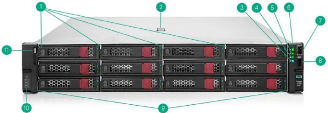
Front View - 12LFF chassis shown
